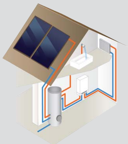
Integrated solar DHW heating system using a Vitocell-B 100 dual-coil storage tank
