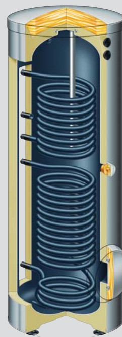
Vitocell-B 100 dual-coil storage tank
